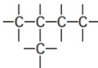
2-Methylbutan
