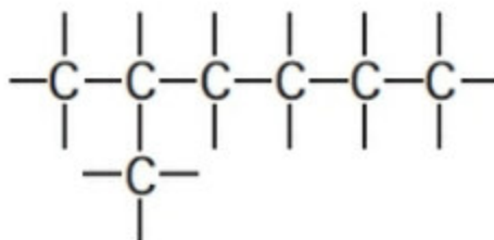
2-Methylhexan
