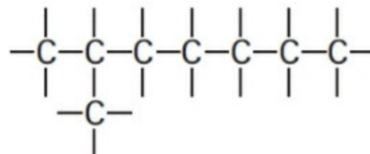
2-Methylheptan
