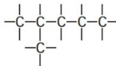
2-Methylpentan
